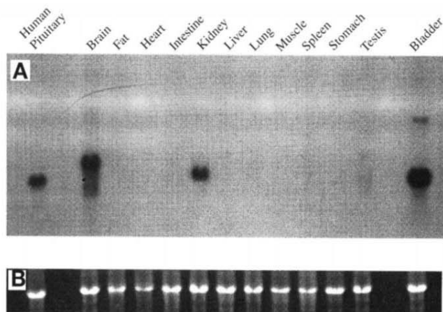
Figure 1. Northern blot analysis of RNA extracted from various tissues of male mice from line GHP2. The blot was probed with ^{32}\text{P} -labeled hGH cDNA. (A) The human pituitary lane contained 1 ng of human pituitary poly A + RNA. Other lanes contained 15 \mu\text{g} of total RNA from various tissues, except for the bladder lane, which contained 300 ng of total RNA. (B) Ethidium bromide staining of the 18S ribosomal RNA subunit.
